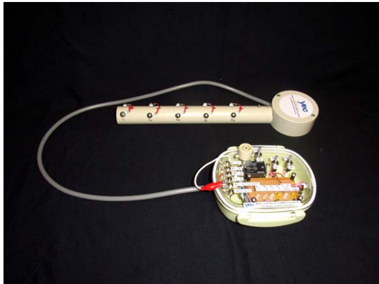
Rainfall Monitoring & Warning System (簡易雨量監視警報裝置)
