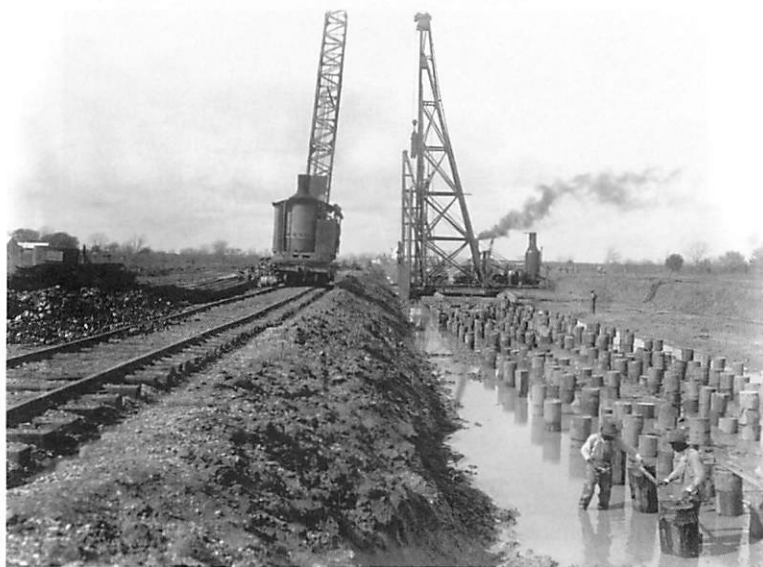
Thousands of wooden pilings were driven to provide a reliable foundation for the spillway structure.
