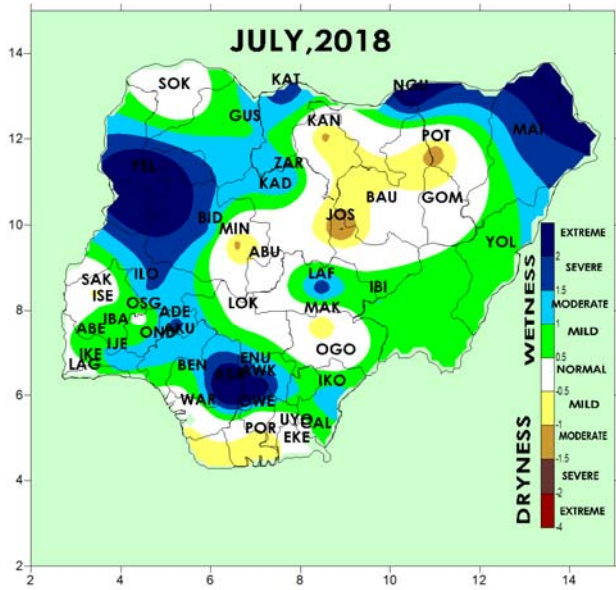
Fig.1: 1-Month Standardized Precipitation Index (for meteorological drought)
